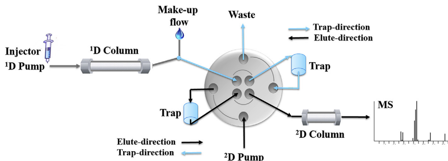
Fig. 8. Schematic illustration of the actively modulated HPLC \times UPLC ( a \times m ) set-up, used in our study.
